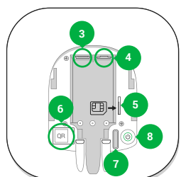
3 - Power supply cable socket 4 - Ethernet cable socket 5 - Micro-SIM card slot 6 - QR code 7 - Tamper button 8 - Power button
